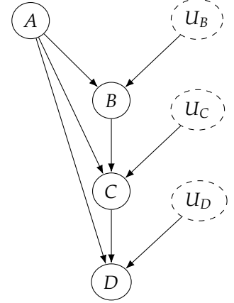
Figure 4.8: Graph for the structural equations in Equation 4.24.
