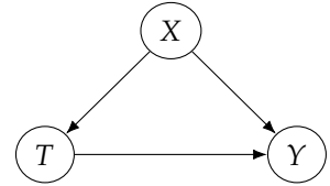
Figure 4.5: Simple causal structure where X counfounds the effect of T on Y and where X is the only confounder.
