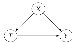
Figure 4.9: Basic causal graph
