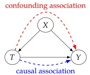
Figure 3.16: Causal graph depicting an example of how confounding association and causal association flow.
