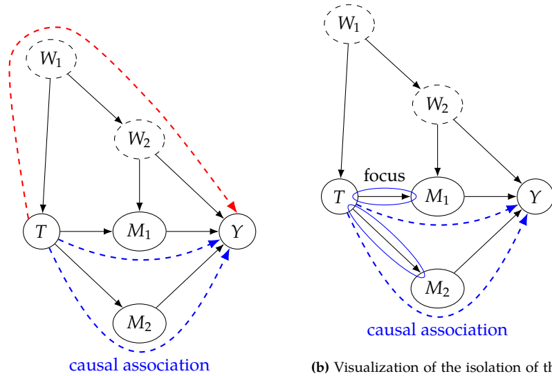
(a) Visualization of the flow of confounding association and causal association.
