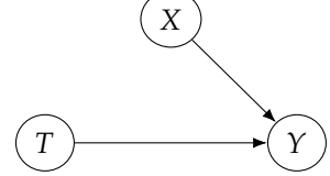
Figure 4.10: Basic causal with the incoming edges to T removed, due to the intervention do(T = t) .
