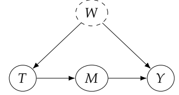
Figure A.1: Causal graph where W is unobserved, so we cannot block the backdoor path T \leftarrow W \rightarrow Y .
